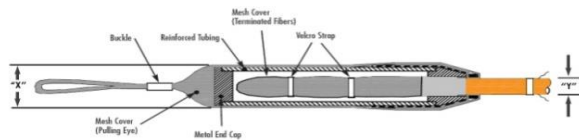
Encapsulated Protection Sleeve
